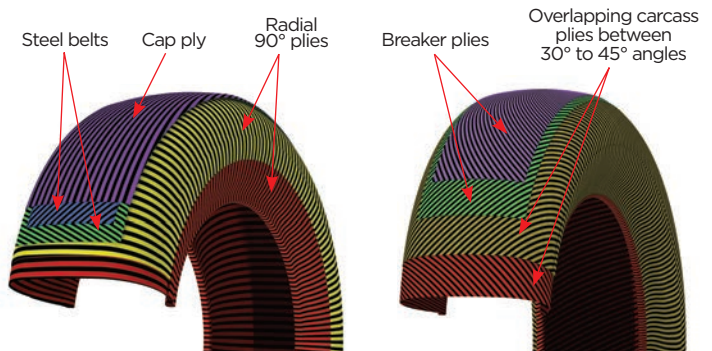
Radial Tire Construction
